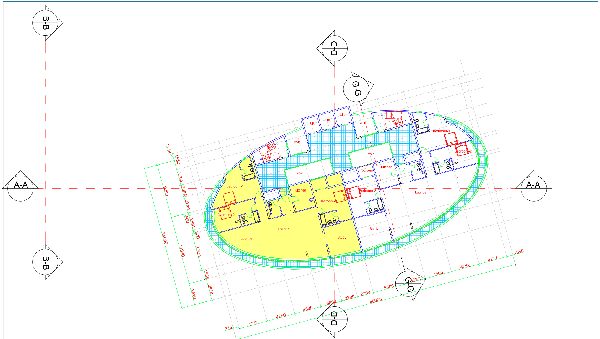
TYPICAL PENTHOUSE FLOOR PLAN LEVELS 17 - 18 : VMP FLATS - 2 2 No 3 - Bedroom Flats ( area - 278msq x 2 = 556msq)
